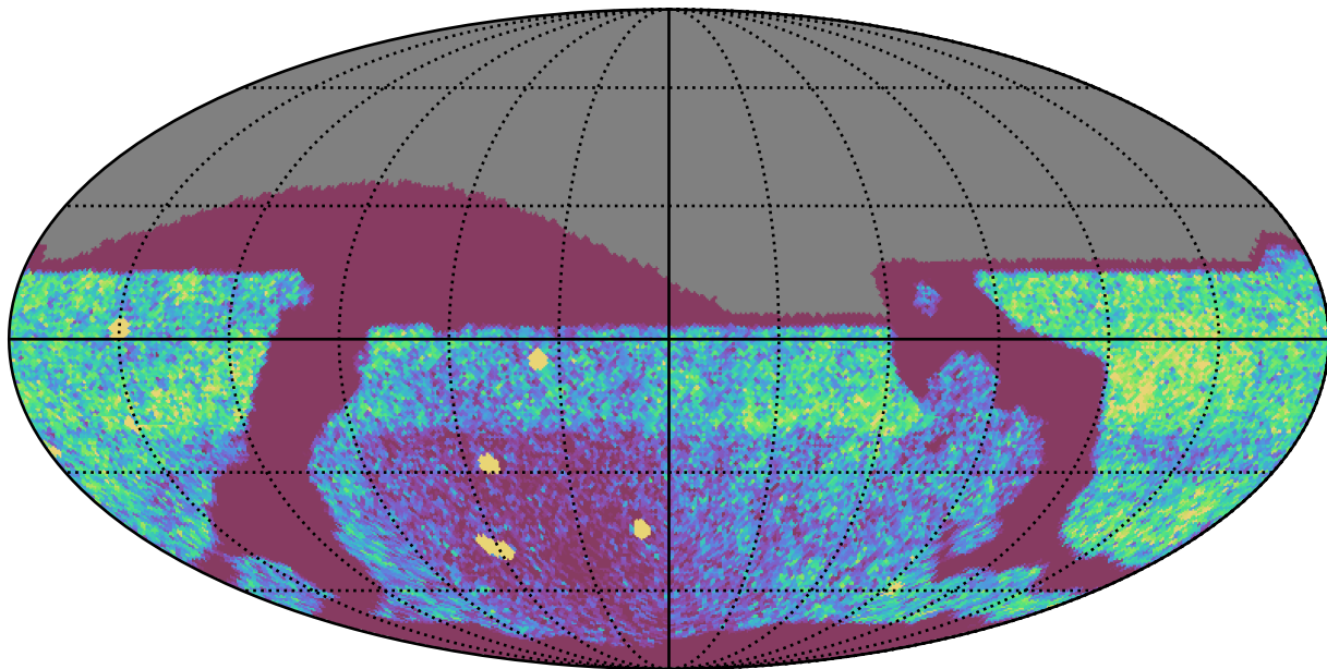
early_u_fpextra4.0_v3.4_10yrs Yr 1 all bands: NVisits
