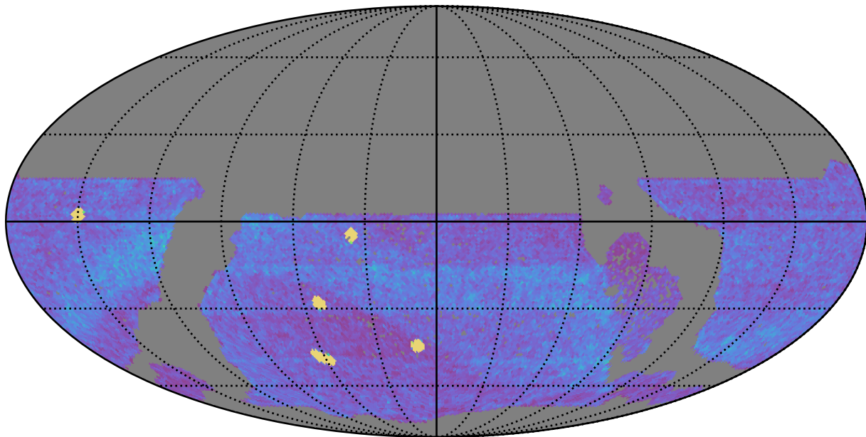
early_u_fpextra4.0_v3.4_10yrs WFD all bands: NVisits
