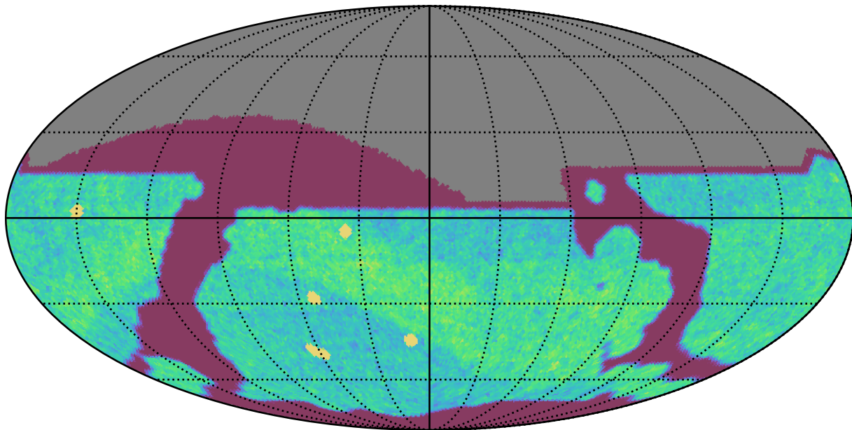
early_u_fpextra4.0_v3.4_10yrs All sky i band: NVisits
