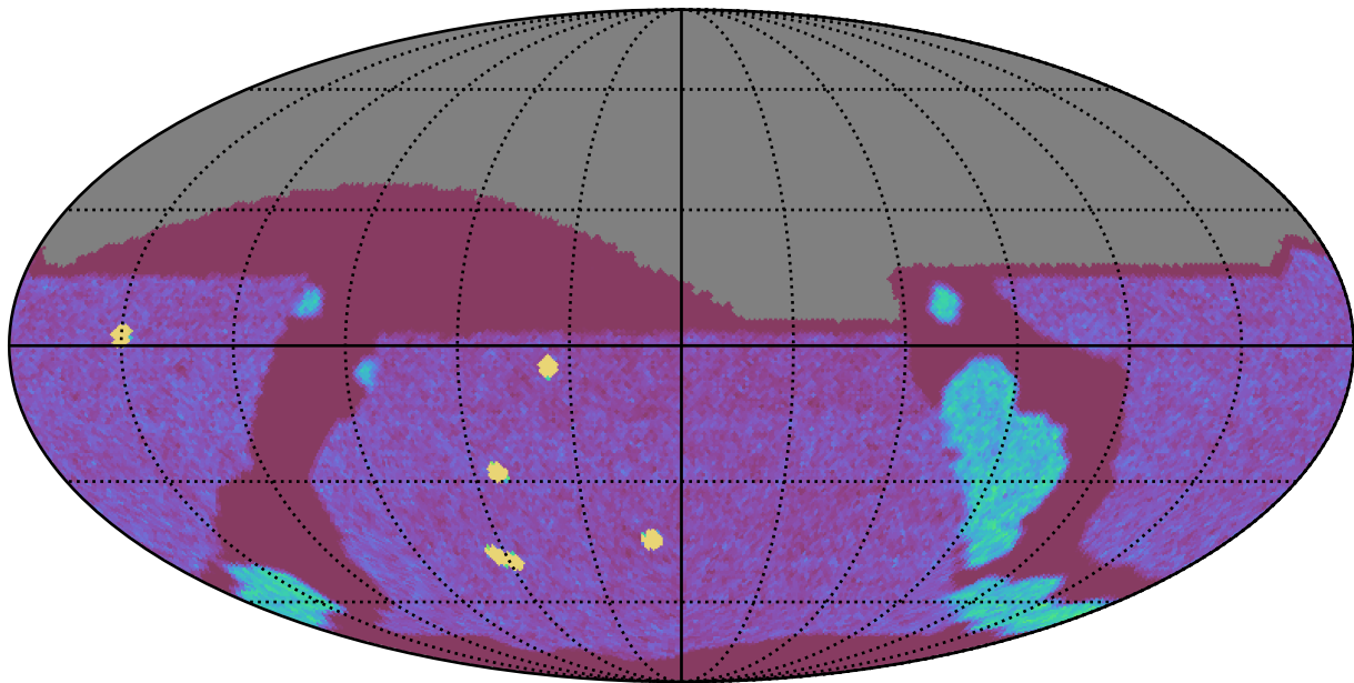
early_u_fpextra4.0_v3.4_10yrs All sky g band: NVisits
