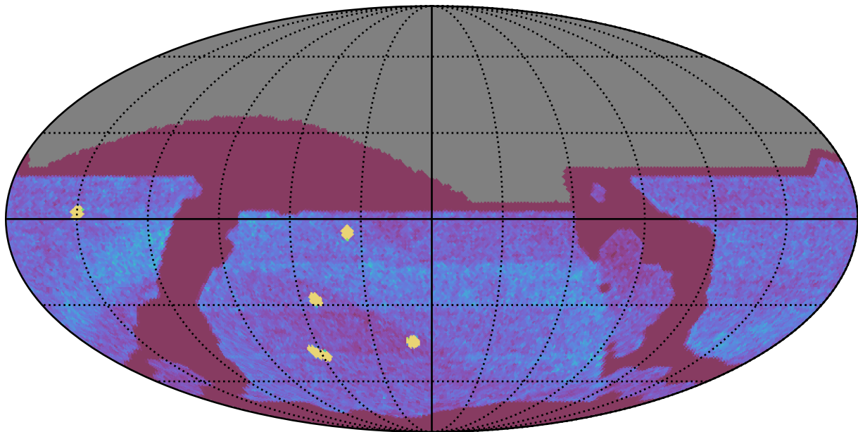
early_u_fpextra4.0_v3.4_10yrs All sky all bands: NVisits
