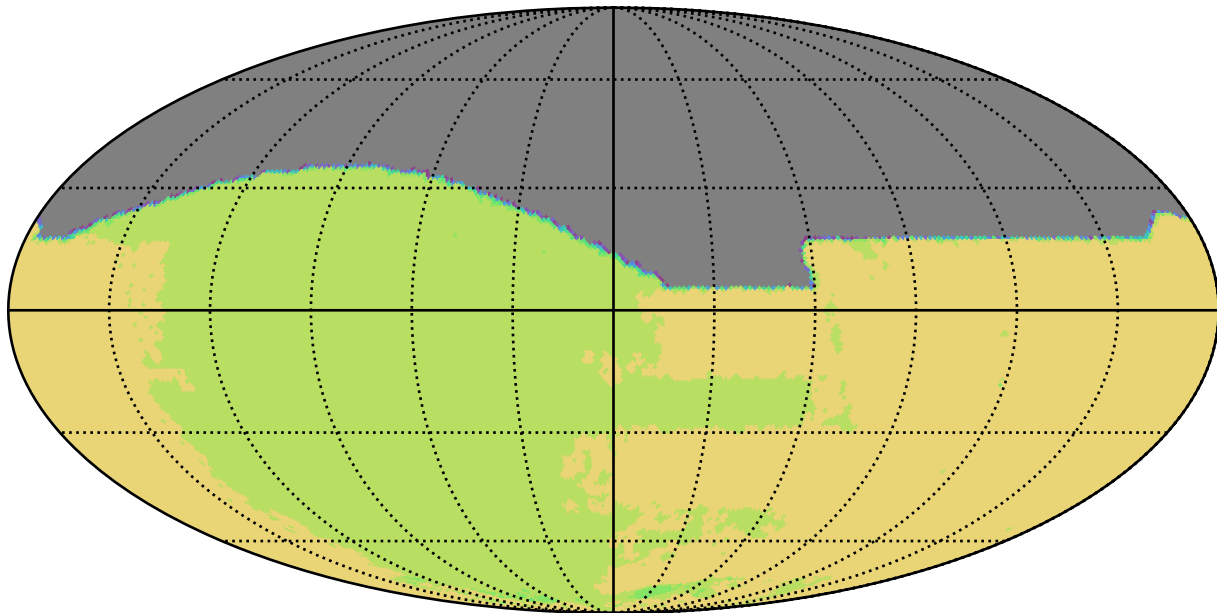
early_u_fpextra4.0_v3.4_10yrs All sky all bands: NSeasons
