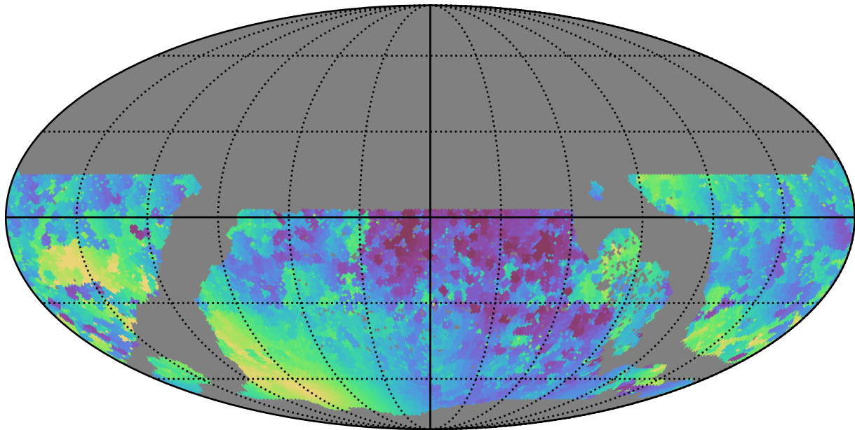
early_u_fpextra4.0_v3.4_10yrs WFD y band: Min solarElong
