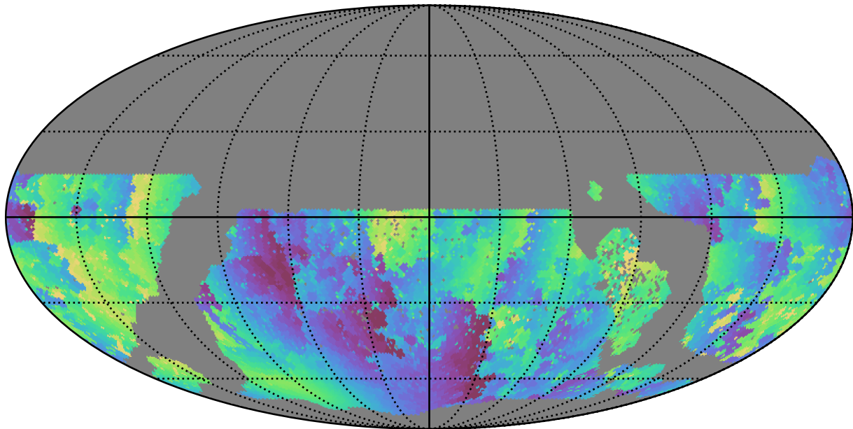
early_u_fpextra4.0_v3.4_10yrs WFD u band: Min solarElong
