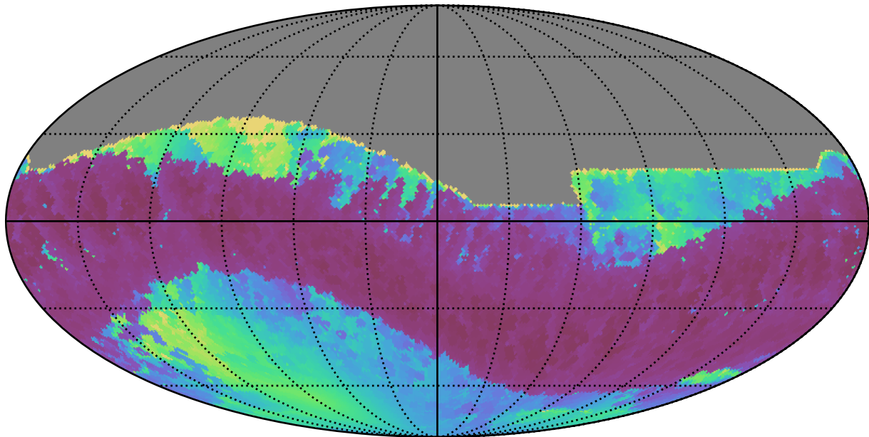
early_u_fpextra4.0_v3.4_10yrs All sky z band: Min solarElong
