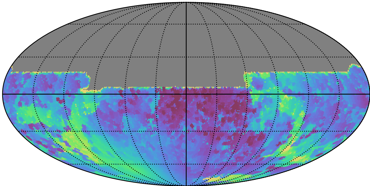
early_u_fpextra4.0_v3.4_10yrs All sky y band: Min solarElong
