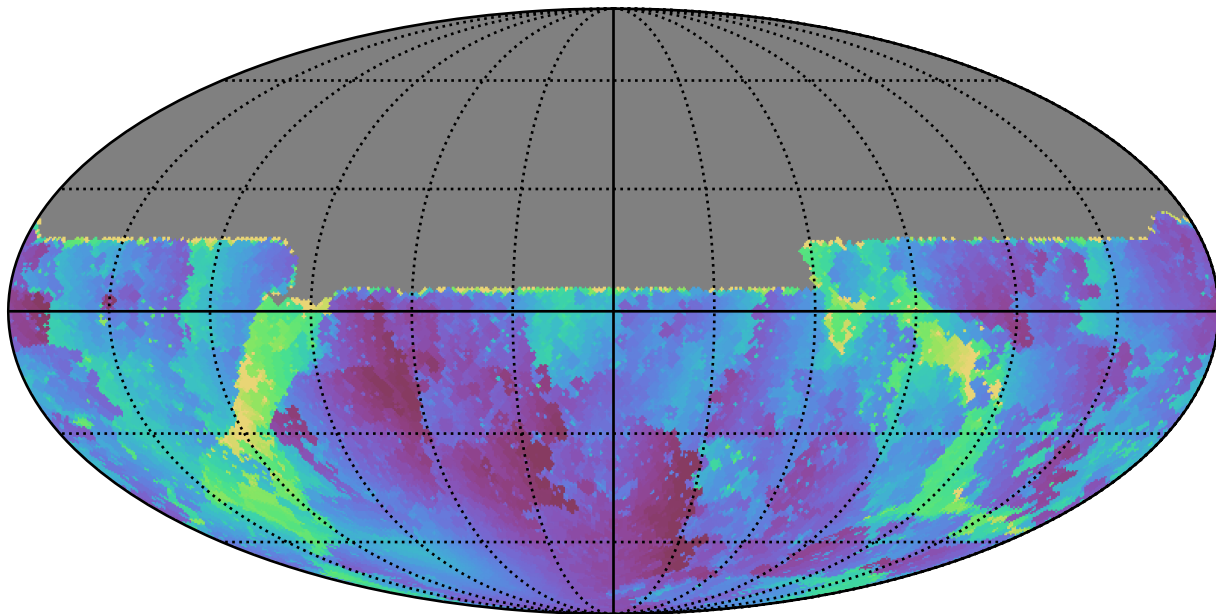
early_u_fpextra4.0_v3.4_10yrs All sky u band: Min solarElong
