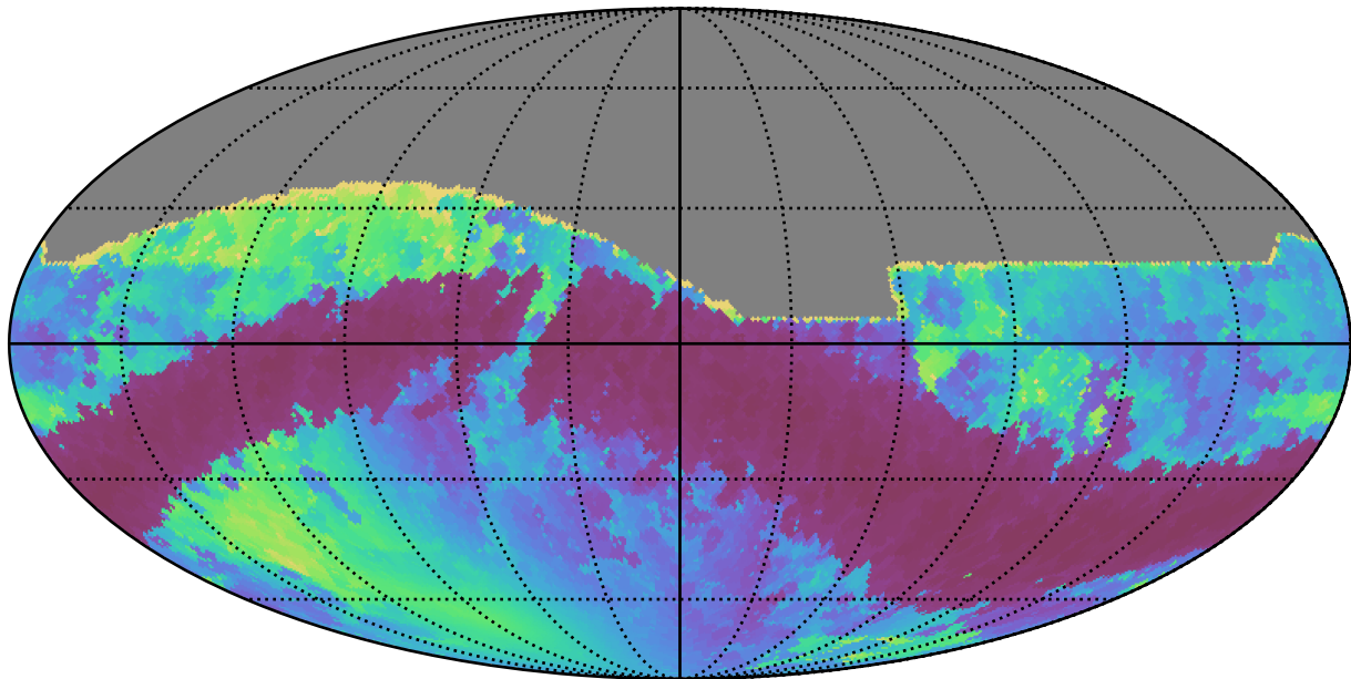
early_u_fpextra4.0_v3.4_10yrs All sky r band: Min solarElong
