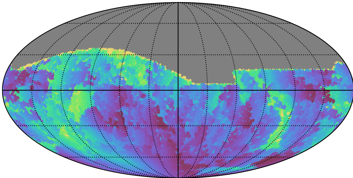
early_u_fpextra4.0_v3.4_10yrs All sky g band: Min solarElong
