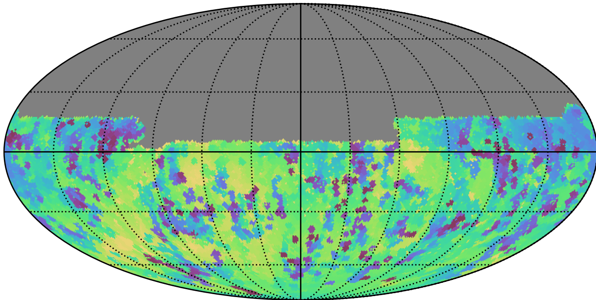
early_u_fpextra4.0_v3.4_10yrs Yr 1 y band: Min skyBrightness
