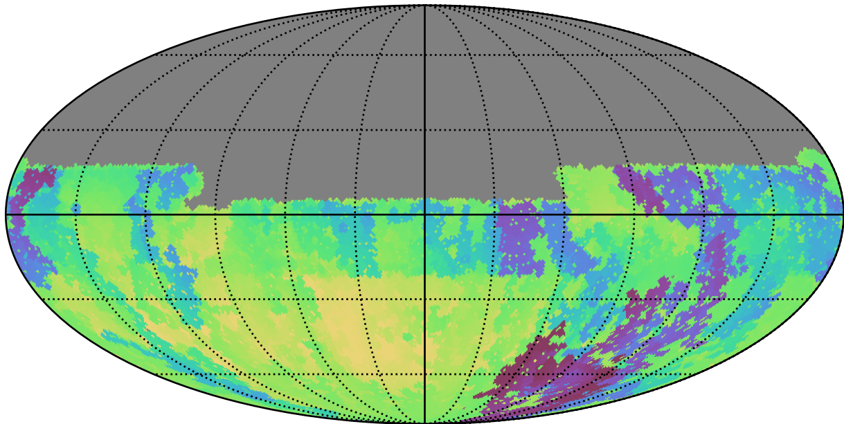
early_u_fpextra4.0_v3.4_10yrs Yr 1 u band: Min skyBrightness
