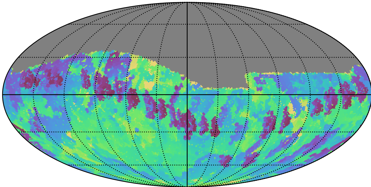
early_u_fpextra4.0_v3.4_10yrs Yr 1 i band: Min skyBrightness
