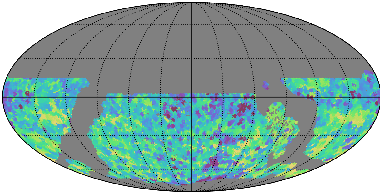
early_u_fpextra4.0_v3.4_10yrs WFD y band: Min skyBrightness
