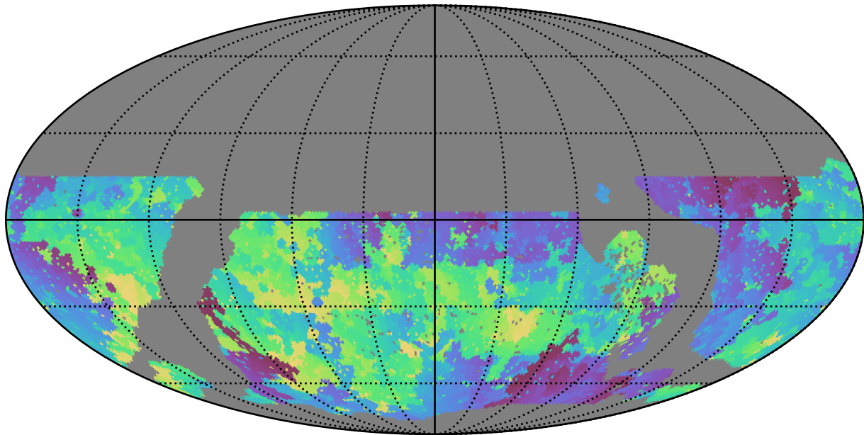
early_u_fpextra4.0_v3.4_10yrs WFD u band: Min skyBrightness
