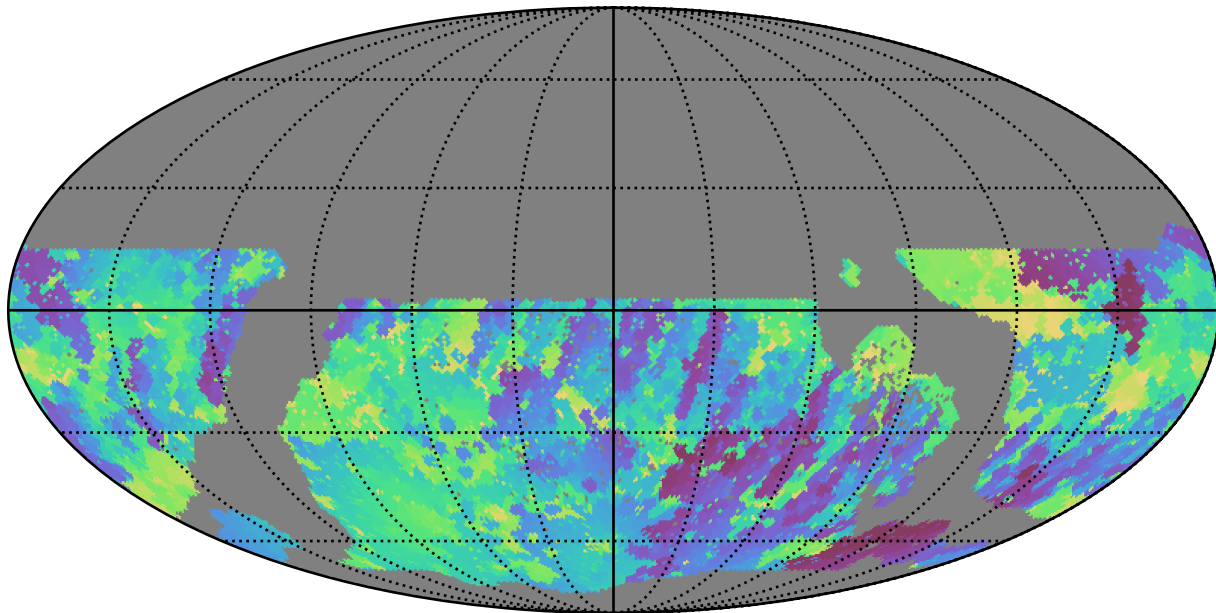
early_u_fpextra4.0_v3.4_10yrs WFD r band: Min skyBrightness
