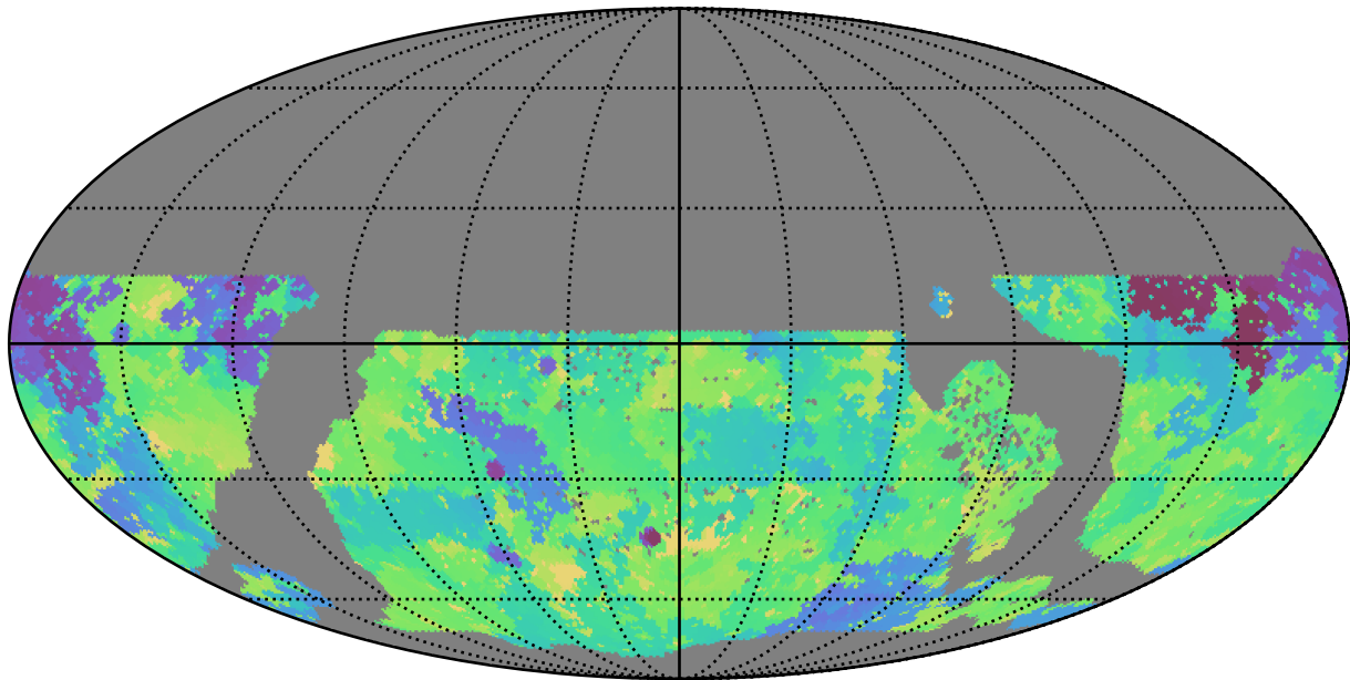
early_u_fpextra4.0_v3.4_10yrs WFD g band: Min skyBrightness
