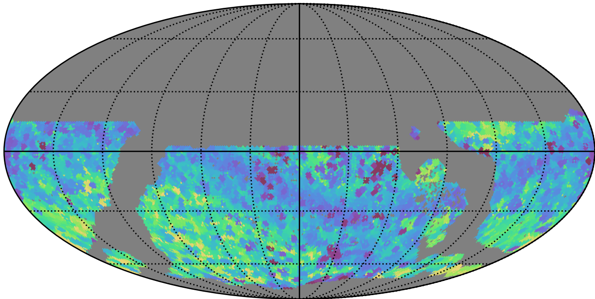
early_u_fpextra4.0_v3.4_10yrs WFD all bands: Min skyBrightness
