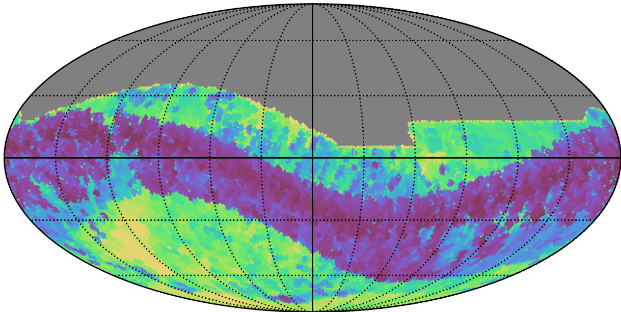
early_u_fpextra4.0_v3.4_10yrs All sky z band: Min skyBrightness
