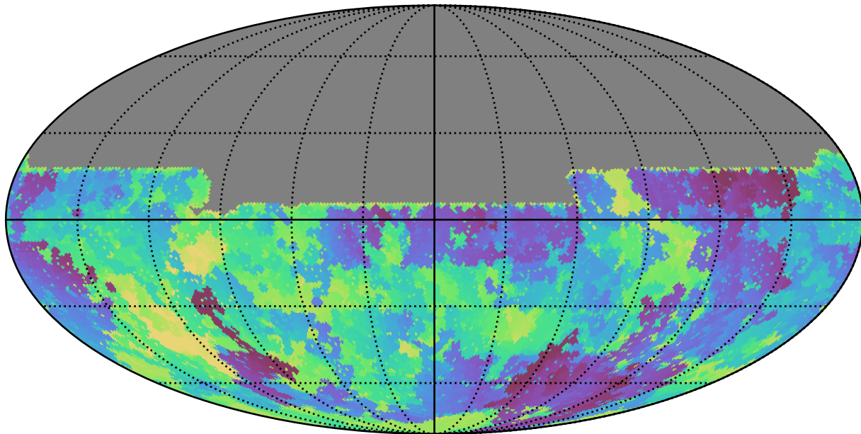
early_u_fpextra4.0_v3.4_10yrs All sky u band: Min skyBrightness
