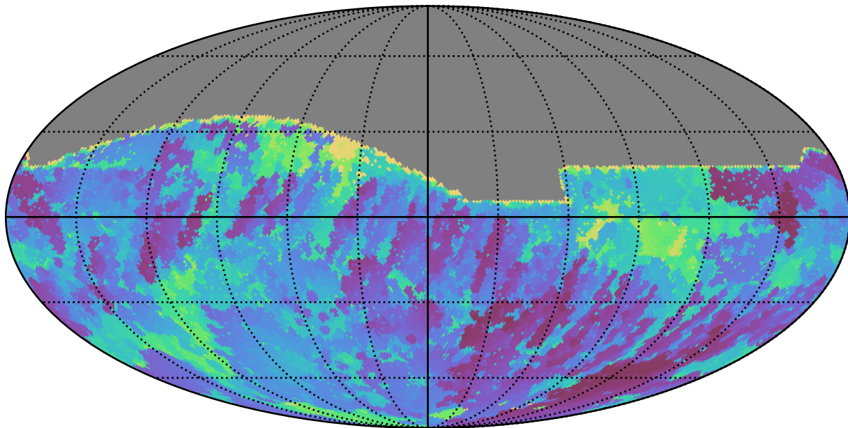
early_u_fpextra4.0_v3.4_10yrs All sky r band: Min skyBrightness
