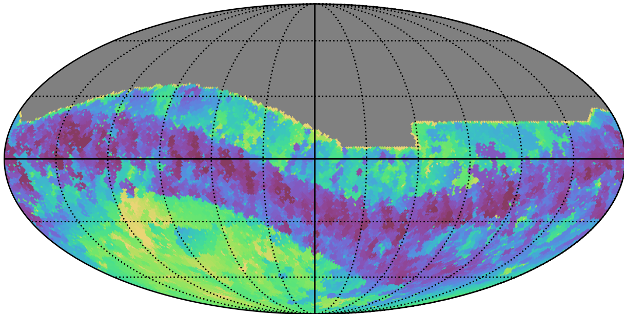
early_u_fpextra4.0_v3.4_10yrs All sky i band: Min skyBrightness
