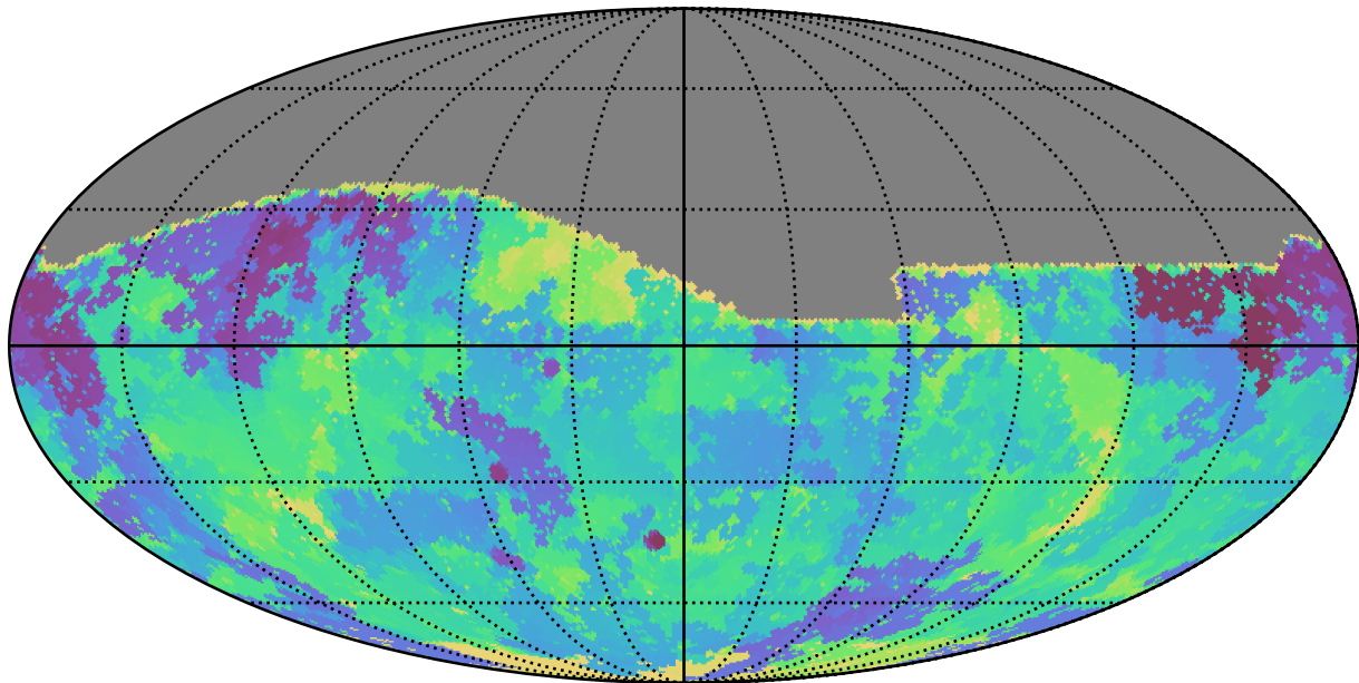
early_u_fpextra4.0_v3.4_10yrs All sky g band: Min skyBrightness
