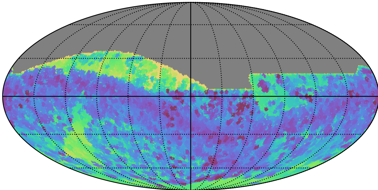
early_u_fpextra4.0_v3.4_10yrs All sky all bands: Min skyBrightness
