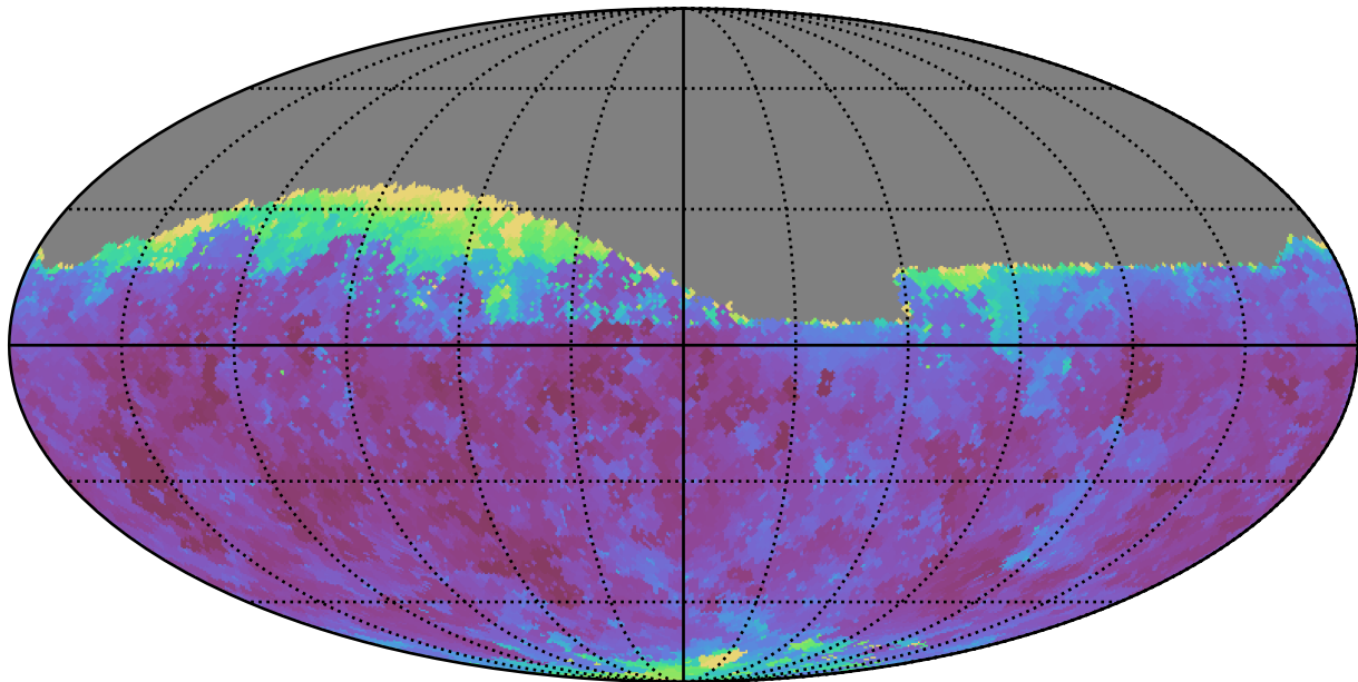
early_u_fpextra4.0_v3.4_10yrs Yr 1 r band: Min seeingGeom
