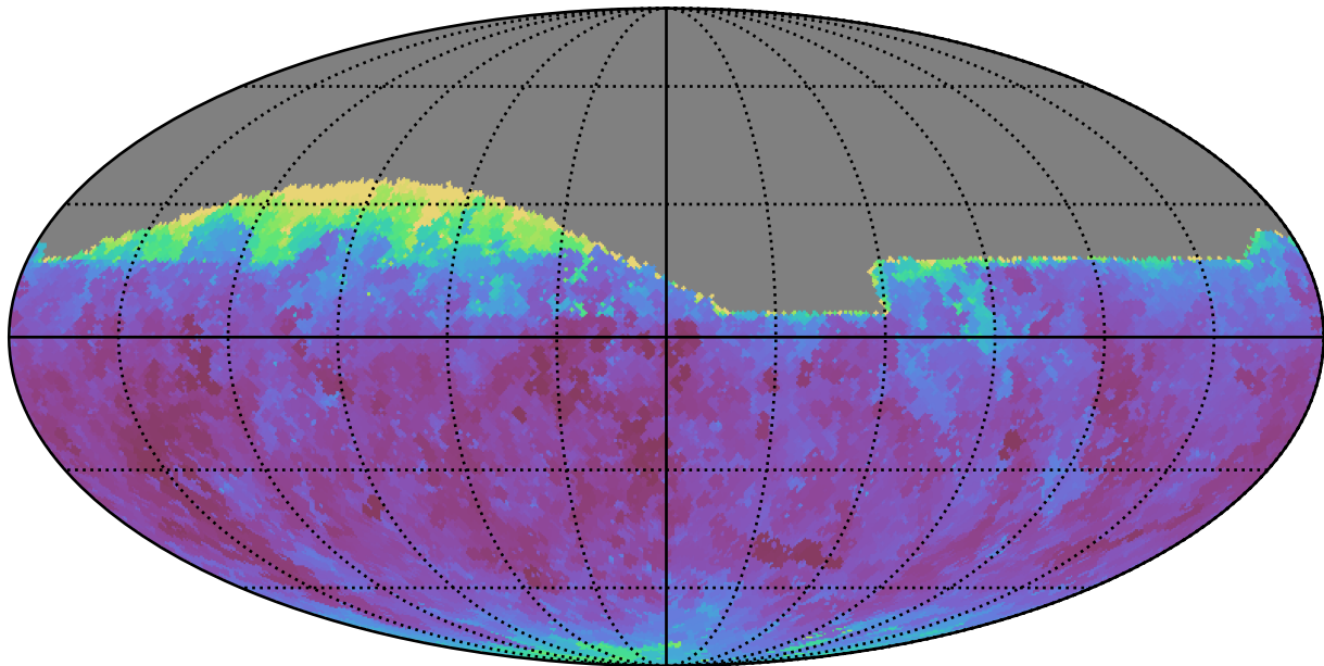
early_u_fpextra4.0_v3.4_10yrs Yr 1 all bands: Min seeingGeom
