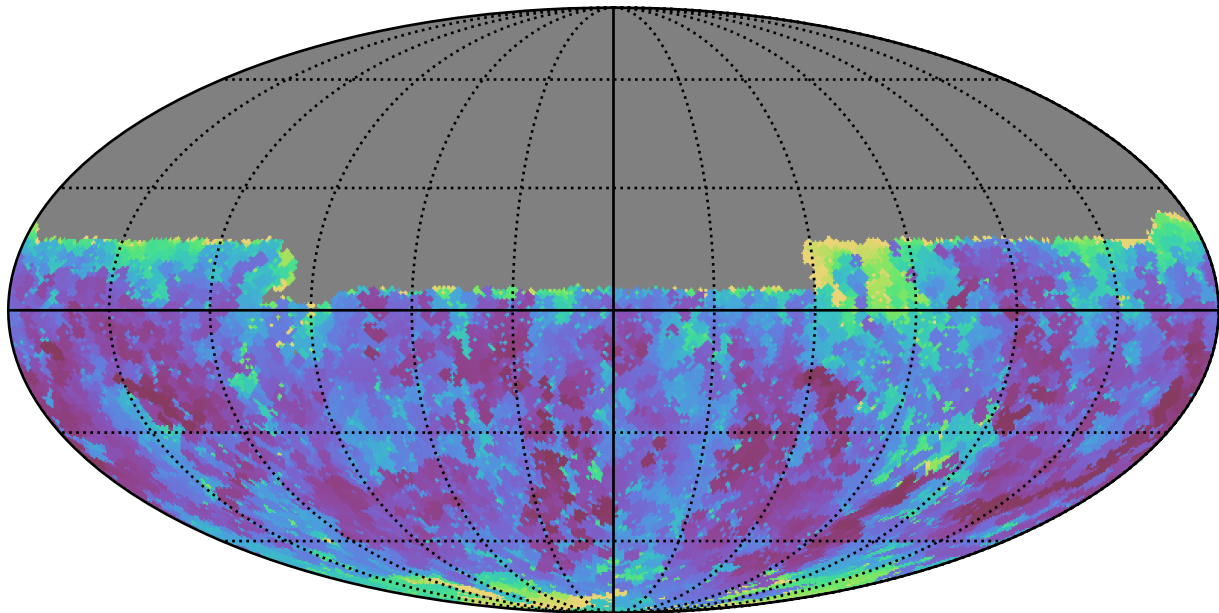
early_u_fpextra4.0_v3.4_10yrs Yr 1 y band: Min seeingEff
