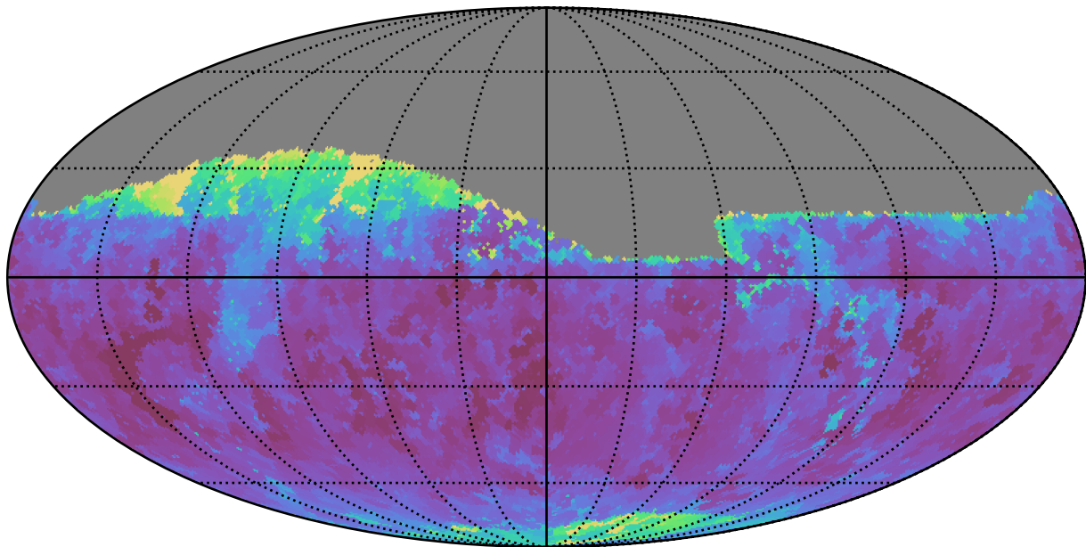
early_u_fpextra4.0_v3.4_10yrs Yr 1 i band: Min seeingEff
