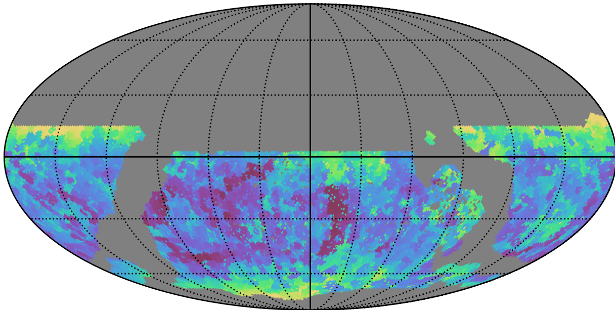
early_u_fpextra4.0_v3.4_10yrs WFD y band: Min seeingEff
