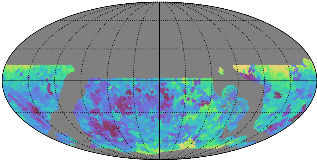
early_u_fpextra4.0_v3.4_10yrs WFD r band: Min seeingEff
