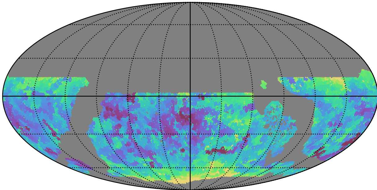
early_u_fpextra4.0_v3.4_10yrs WFD g band: Min seeingEff
