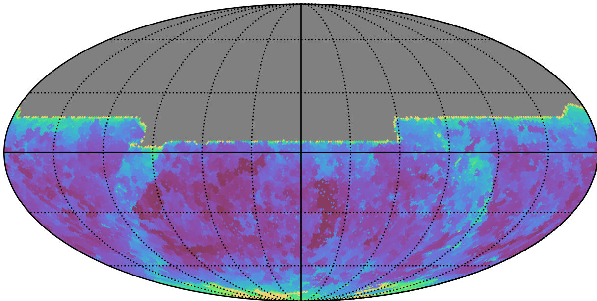
early_u_fpextra4.0_v3.4_10yrs All sky y band: Min seeingEff
