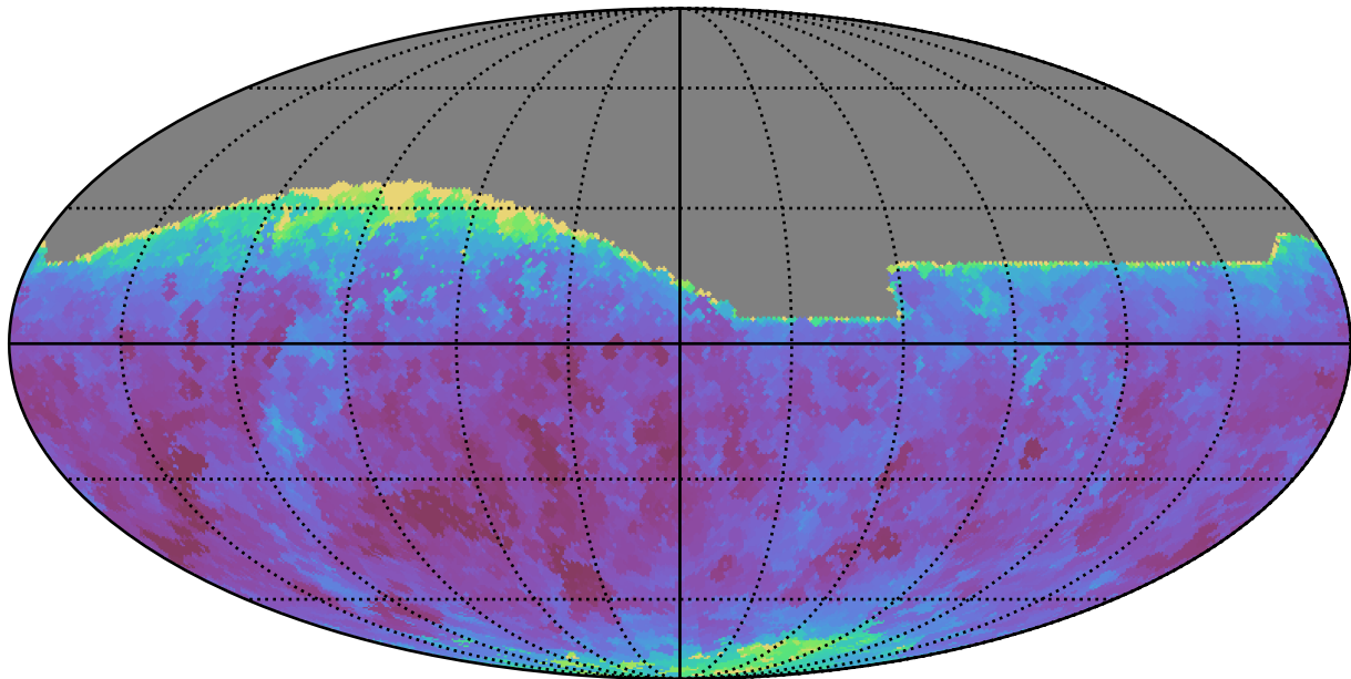
early_u_fpextra4.0_v3.4_10yrs All sky i band: Min seeingEff
