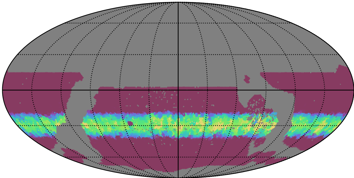
early_u_fpextra4.0_v3.4_10yrs WFD z band: Min normairmass
