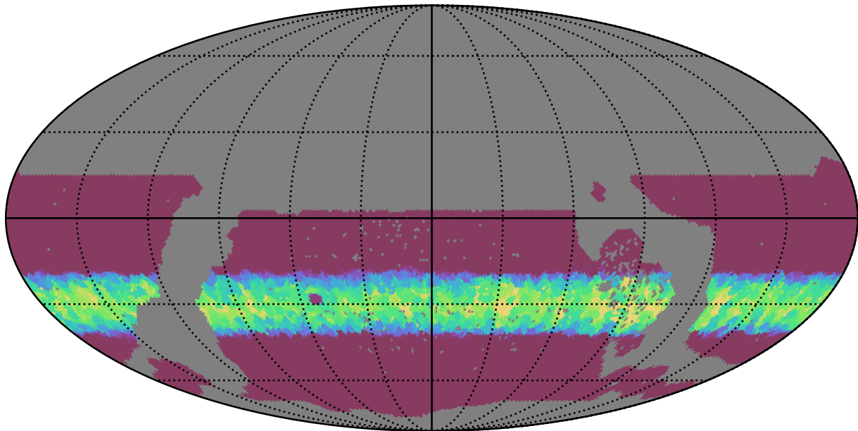
early_u_fpextra4.0_v3.4_10yrs WFD y band: Min normairmass
