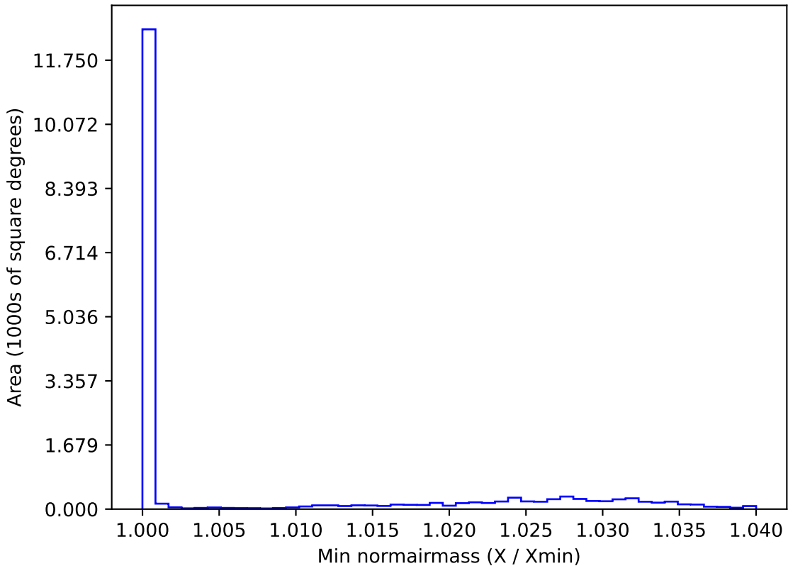
early_u_fpextra4.0_v3.4_10yrs WFD y band: Min normairmass
