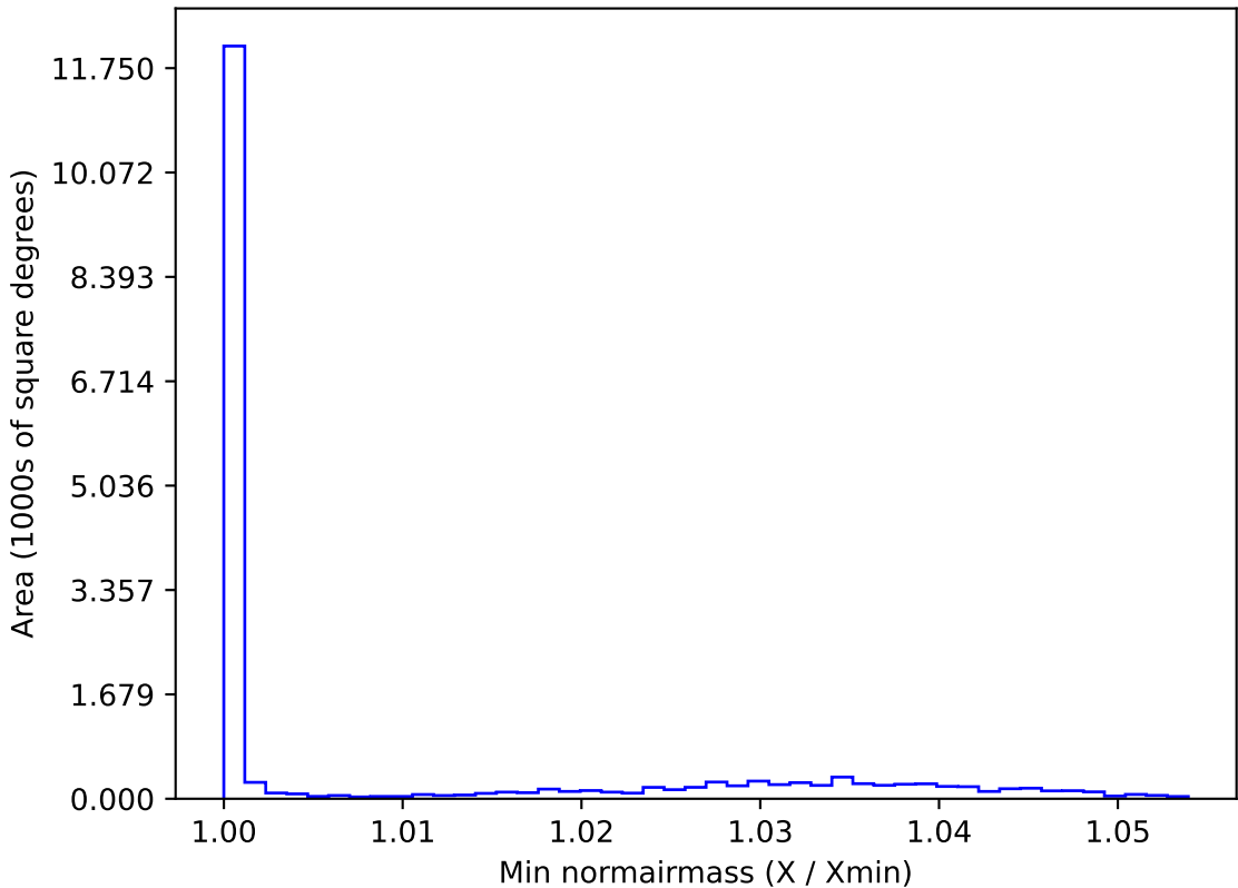
early_u_fpextra4.0_v3.4_10yrs WFD u band: Min normairmass
