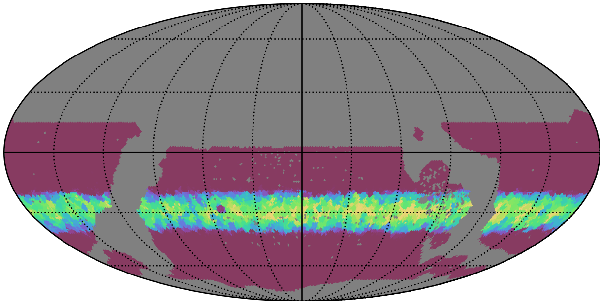
early_u_fpextra4.0_v3.4_10yrs WFD r band: Min normairmass
