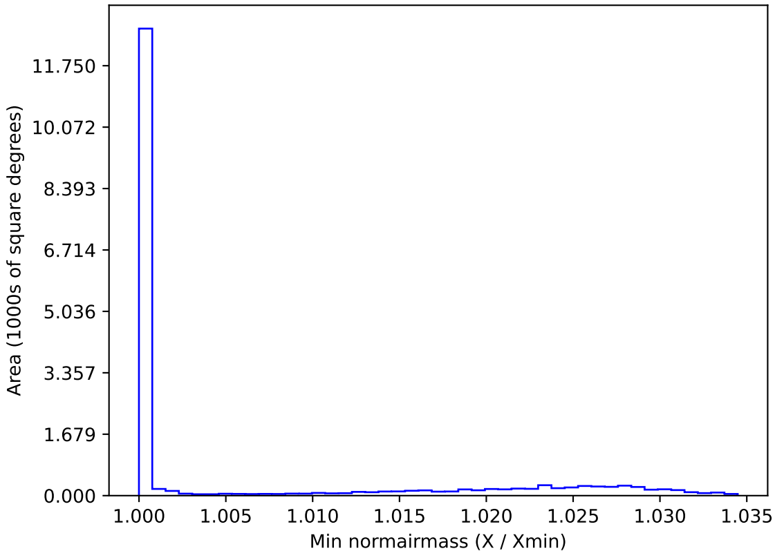
early_u_fpextra4.0_v3.4_10yrs WFD i band: Min normairmass
