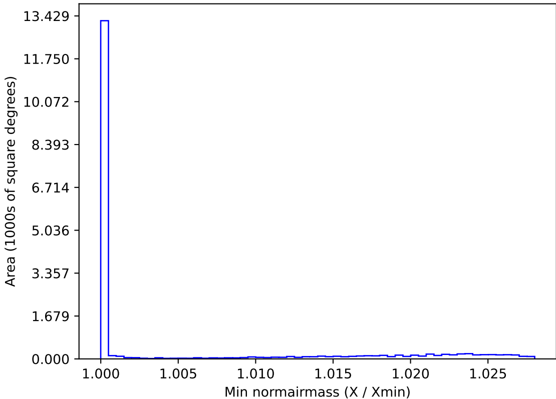
early_u_fpextra4.0_v3.4_10yrs WFD all bands: Min normairmass
