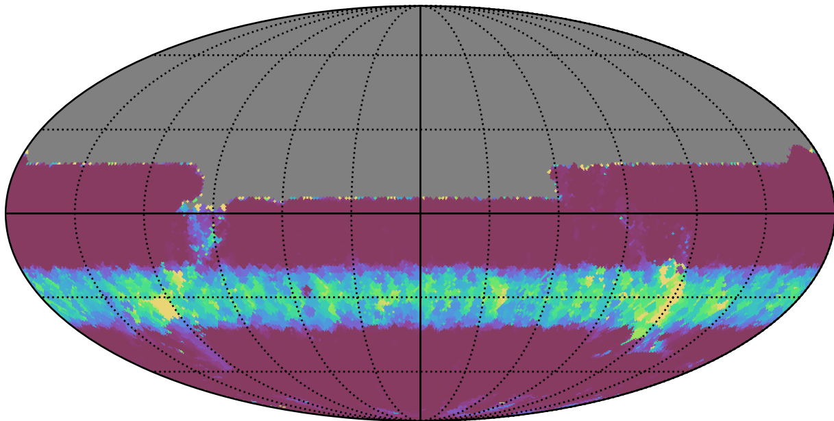
early_u_fpextra4.0_v3.4_10yrs All sky u band: Min normairmass
