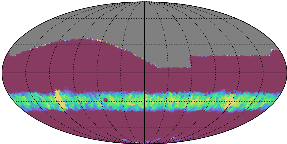
early_u_fpextra4.0_v3.4_10yrs All sky r band: Min normairmass
