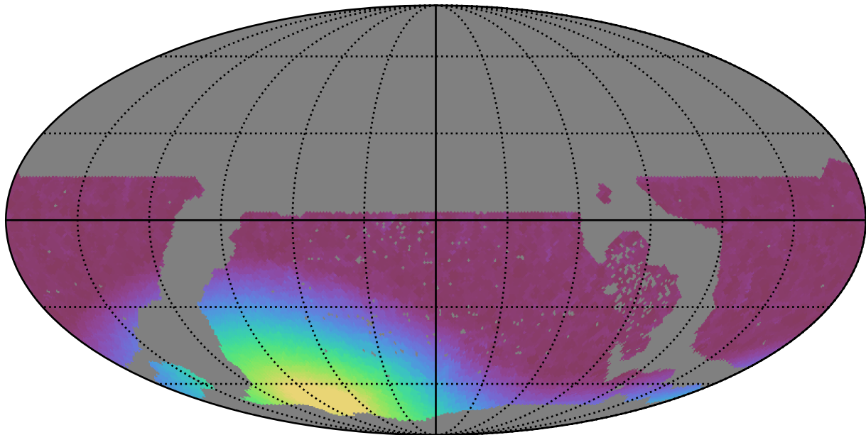
early_u_fpextra4.0_v3.4_10yrs WFD z band: Min moonDistance
