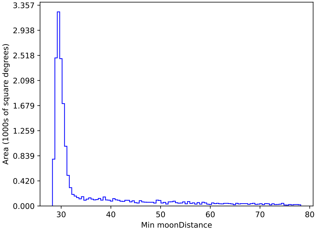
early_u_fpextra4.0_v3.4_10yrs WFD z band: Min moonDistance
