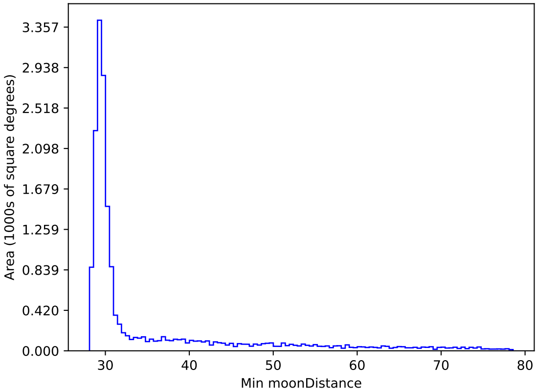
early_u_fpextra4.0_v3.4_10yrs WFD y band: Min moonDistance
