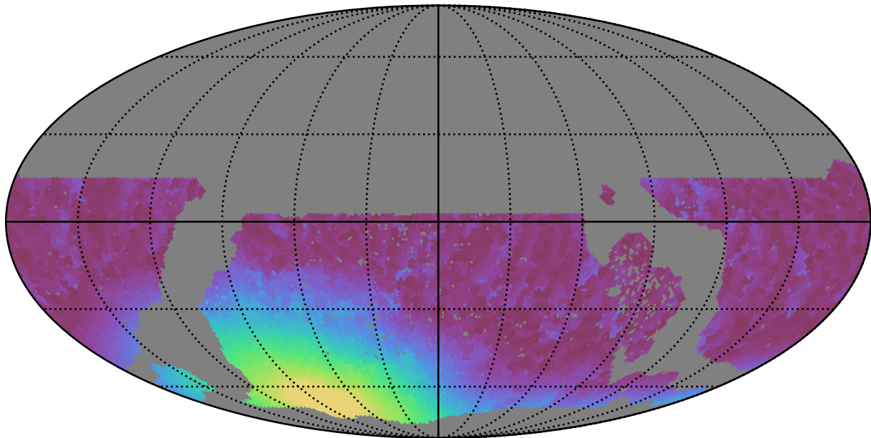
early_u_fpextra4.0_v3.4_10yrs WFD r band: Min moonDistance
