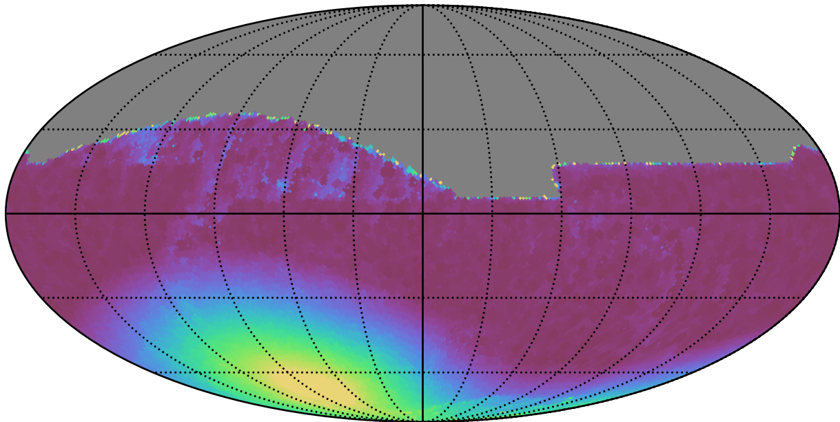
early_u_fpextra4.0_v3.4_10yrs All sky z band: Min moonDistance
